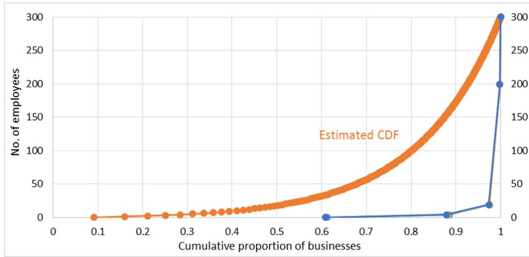
Figure 2-2 Estimated CDF #1 and CDF data point comparison, Australia, 2011/12 - 2013/14
