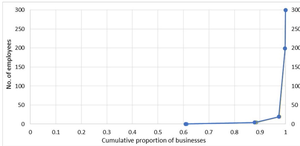
Figure 2-1 Cumulative distribution function data point plot, Australia, 2011/12 - 2013/14 a
